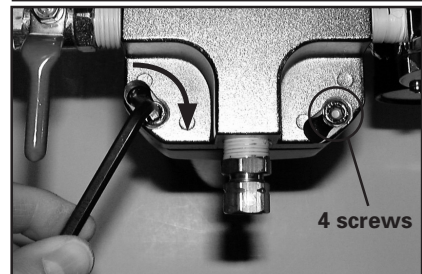
12. Tighten screws tight.
